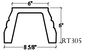
Bottom Rails
